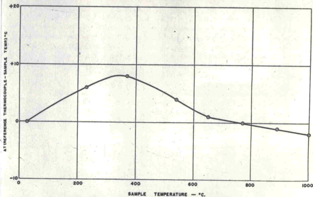
Fig. 5. Typical calibration curve showing difference between temperature of reference thermocouple and sample temperature as measured by thermocouple between piston faces under pressure.
